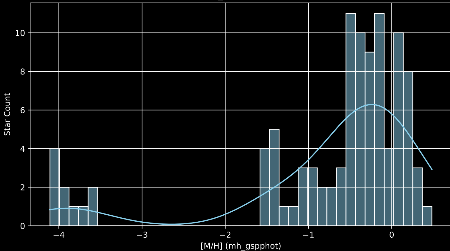
APOGEE DR17 Field: [ORIONA-B [M/H] (mh_gspphot) (n= 101)
