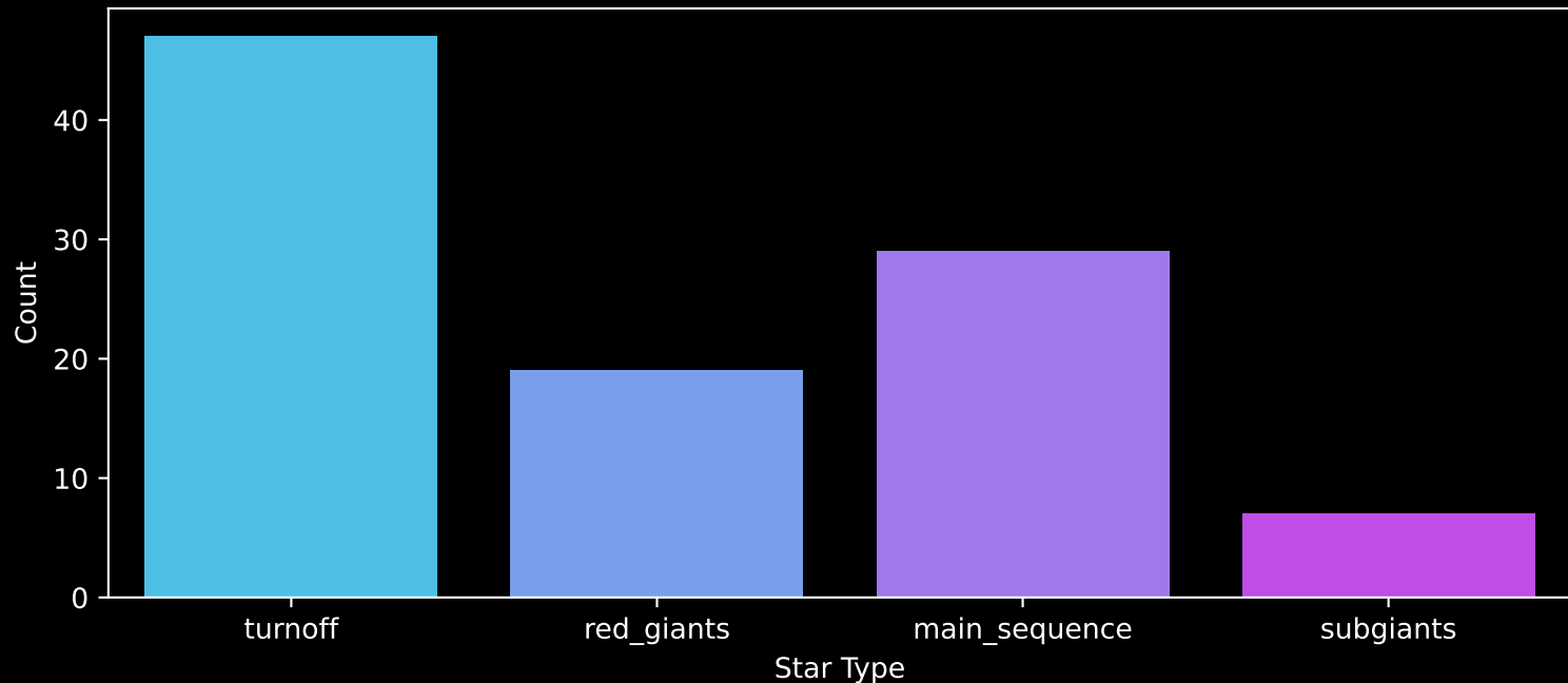
APOGEE DR17 Field: [ORIONA-B] Count plot of Star Type
