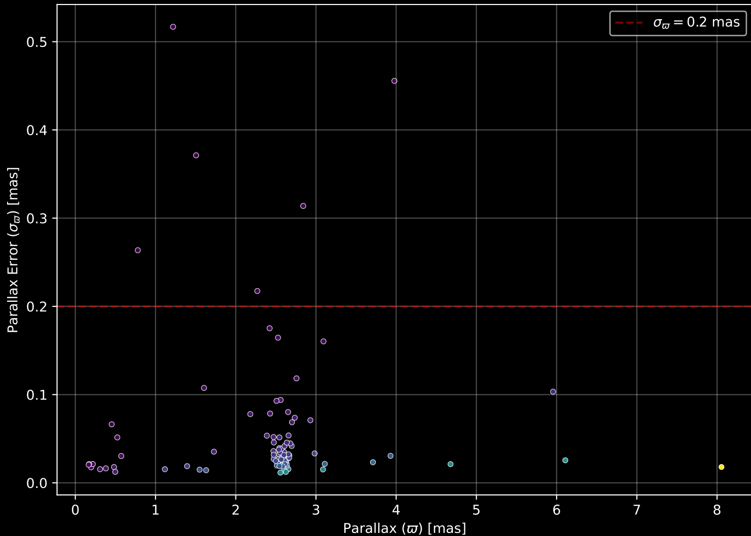
APOGEE DR17 Field: [ORIONA-B] Parallax Quality (n= 102)
