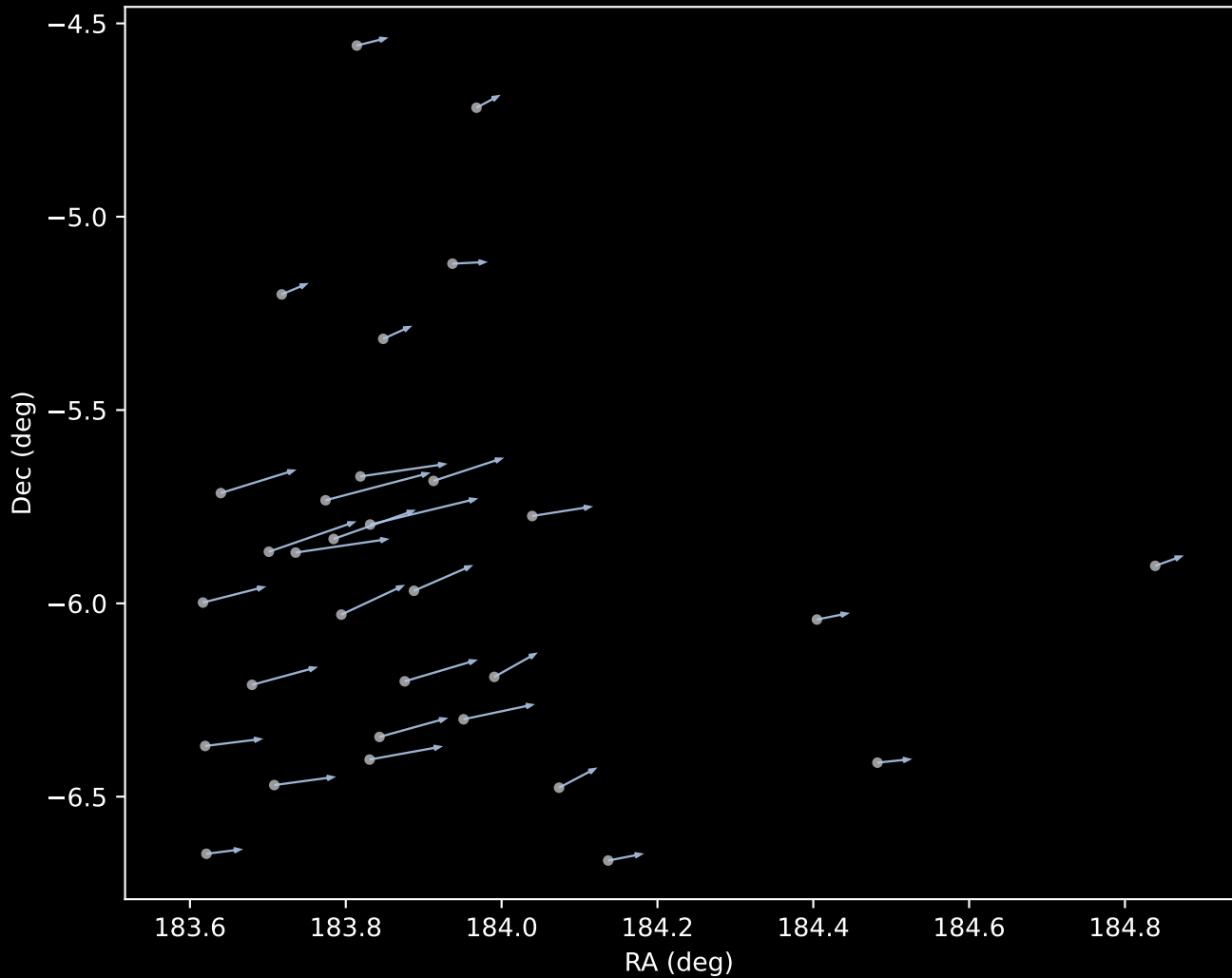
APOGEE DR17 Cluster 1 Proper Motion Vectors (n=31)
