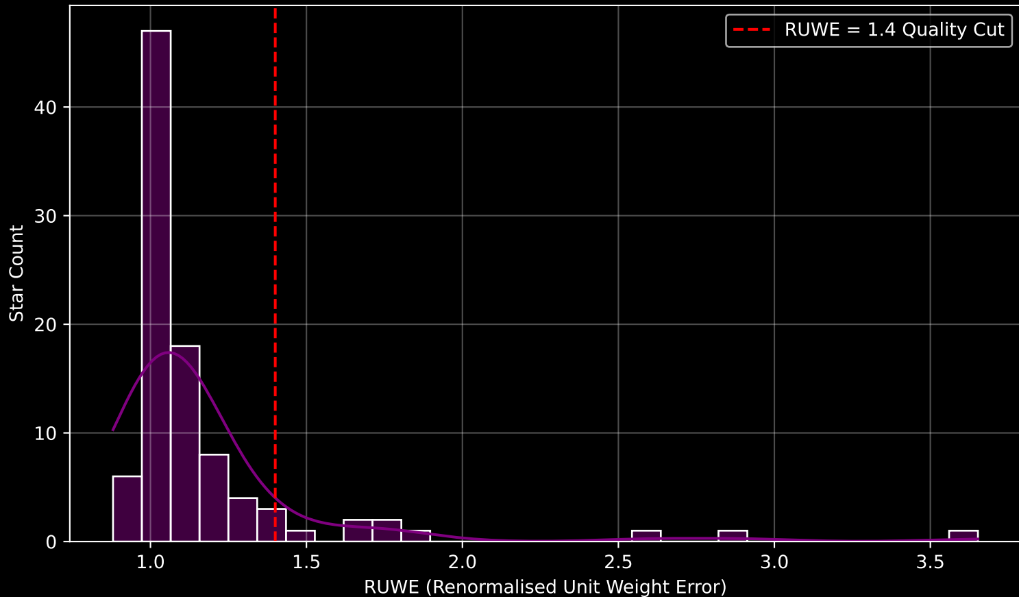
GAPOGEE DR17 Field [ORIONA-B] RUWE Distribution (n= 95)
