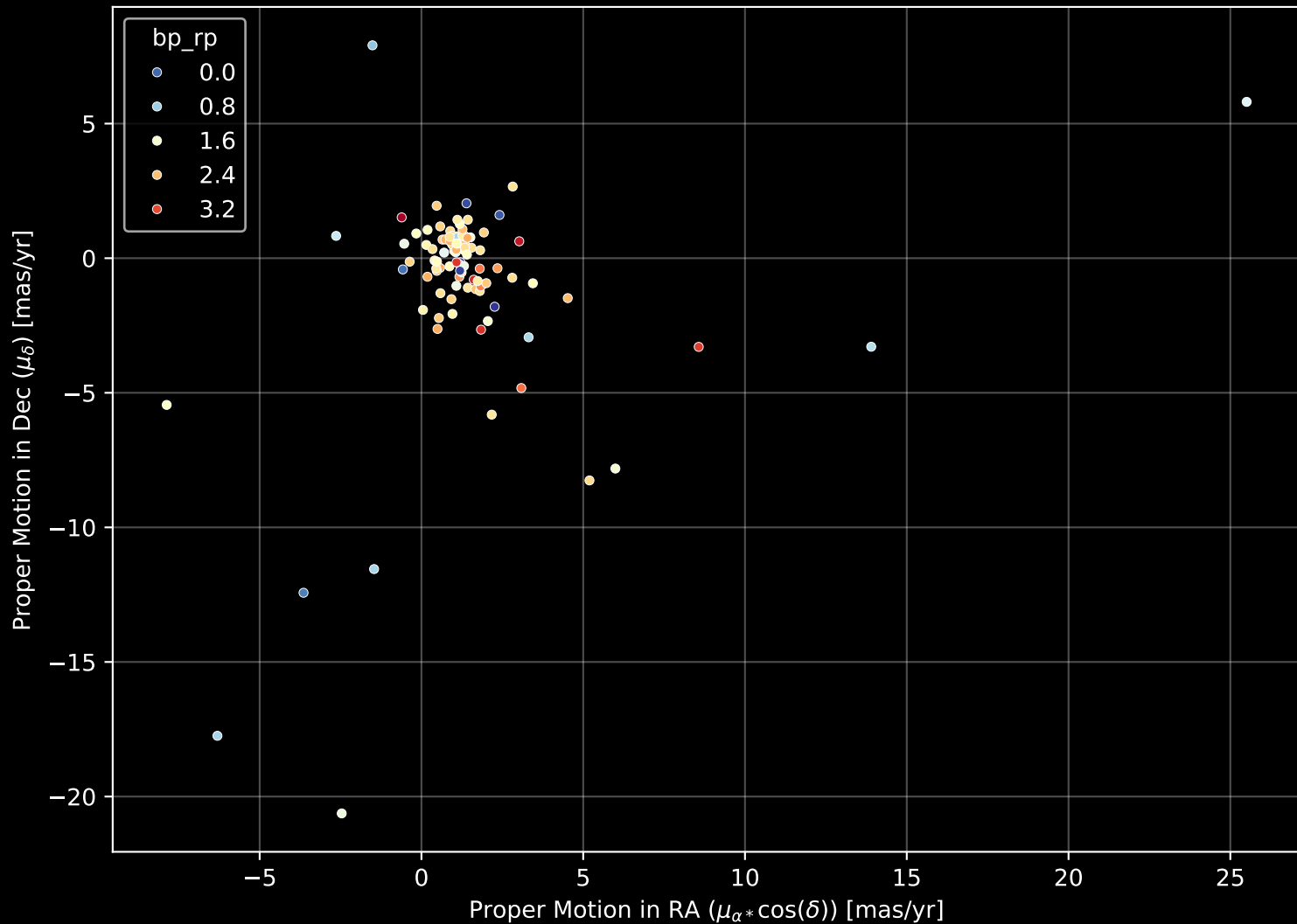
APOGEE DR17 Field: [ORIONA-B] Proper Motion Diagram (n= 102)
